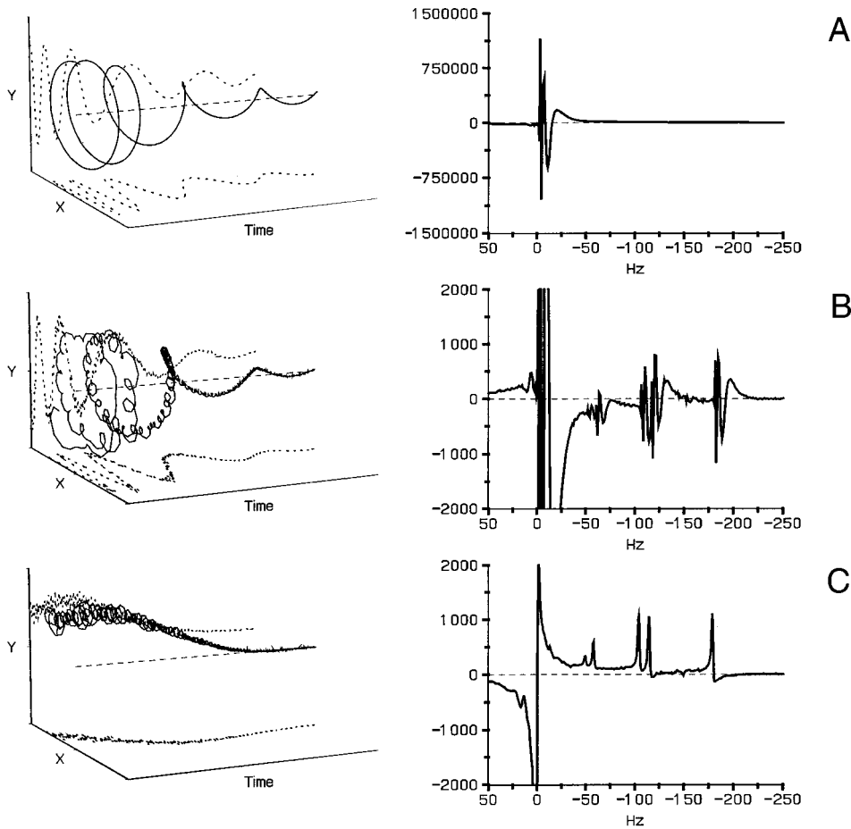
FIG. 12. Post-processing example of eddy current correction (ECC) technique for a PRESS (TE=135,TR=3000) FID from a phantom of pure water and 45 mM methyl protons of NAA, Cr, and Cho. Panel (A) shows the water unsuppressed time domain and absorption signals. Panel (B) shows the water suppressed signals acquired with the water suppression RF pulses switched on. Both (A) and (B) show the same eddy current distortions. Panel (C) was calculated by subtracting the phase of each time domain data point in (A) from the phase of the same time domain data point in (B) (ECC correction). Although ECC automatically gives the correct zero-order phase, some first-order phase correction is still required in panel (C).
