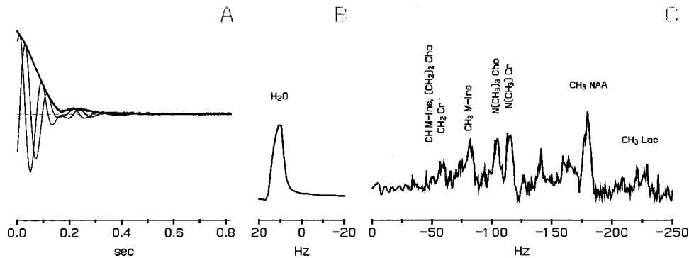
FIG. 8. Example of a bad shim. Panel (A) contains the two received channels (light lines) and the magnitude of the water signal in the time domain. Panel (B) contains the absorption spectrum from the water with a FWHM of 5.6 Hz. Panel (C) shows the absorption spectrum with water suppression. The scaling for the three panels is the same as in Fig. 7.
