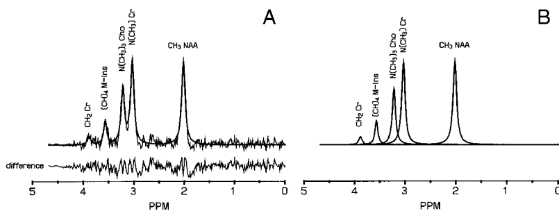
Fig. 17. A demonstration of spectral peak fitting on the baseline corrected in vivo spectrum from Fig. 16 using a nonlinear least-squares method. The heavy solid line in panel (A) shows the fitted spectrum and the lower line is the difference between the raw data and the fitted spectrum. Panel (B) shows the individual peaks from which metabolite areas would be calculated.
