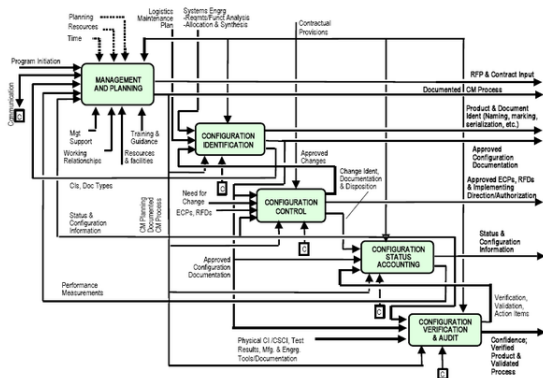
Top level Configuration Management Activity model
